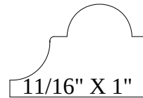
11/16" X 1" RHW H134
