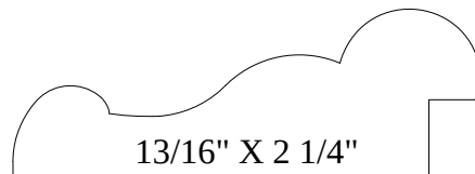
13/16" X 2 1/4" RHW T701
