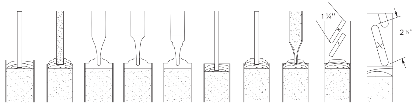
Mission (M) Flat Ovolo (FO) Bladder Pressed (C) Single Hip (H) Double Hip (HD) Mission French Ovolo French Louver Bladder Pressed Panel Standard Louver
